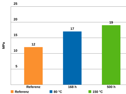
Tensile shear strength after thermal storage, based on DIN EN ISO 527
