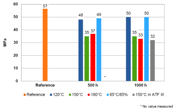
Tensile strength after temperature storage, by the criteria of DIN EN ISO 527 Curing: 1h +80°C
