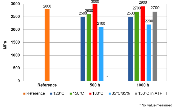
Young's Modulus after temperature storage, by the criteria of DIN EN ISO 527 Curing: 1h +80°C
