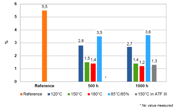
Elongation at tear after temperature storage, by the criteria of DIN EN ISO 527 Curing: 1h +80°C
