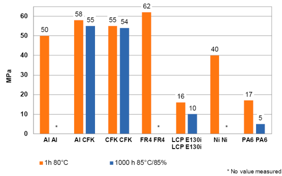
Compression shear strength on different substrates, DELO Standard 5 curing: 1h +80°C
