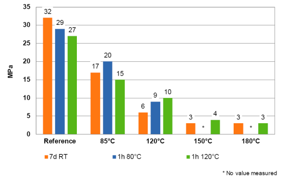
Tensile shear strength measured at the stated temperatures Substrates: Al/Al, by the criteria of DIN EN 1465
