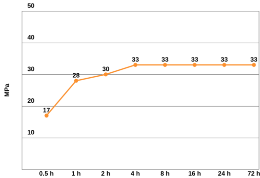
Compression shear strength for determining the curing process shaft-to-hub bonding, substrates: steel shaft/steel hub, based on ISO 10123
