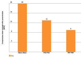
Compression shear strength after preactivation based on DELO Standard 5
