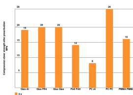
Compression shear strength after preactivation based on DELO Norm 5
