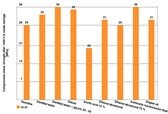
Media resistance after 1000 h
