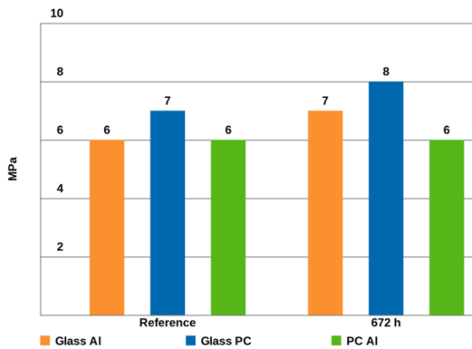
Compression shear strength after temperature storage at, DELO-Norm 5
