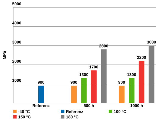
Young's modulus after thermal storage Curing 400 nm 200 mW/cm 2 90 s /
