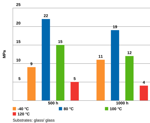
Compression shear strength after thermal storage, based on DELO Standard 5
