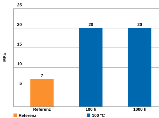
Compression shear strength after thermal storage, based on DELO Standard 5
