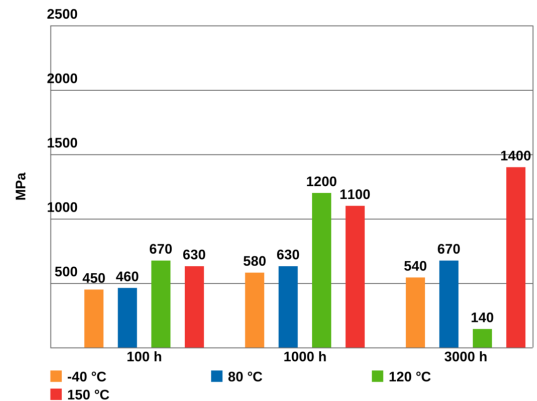
Young's modulus after thermal storage Curing 60 mW/cm² /
